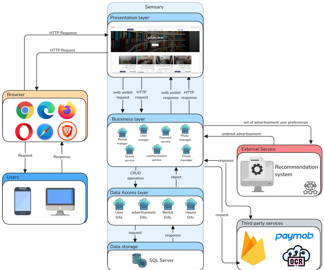
Figure 7: System Architecture diagram
